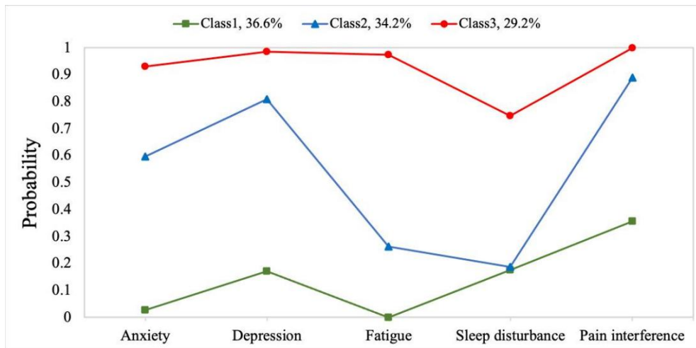
Supplementary Figure 1 The three-class latent profile analysis model
