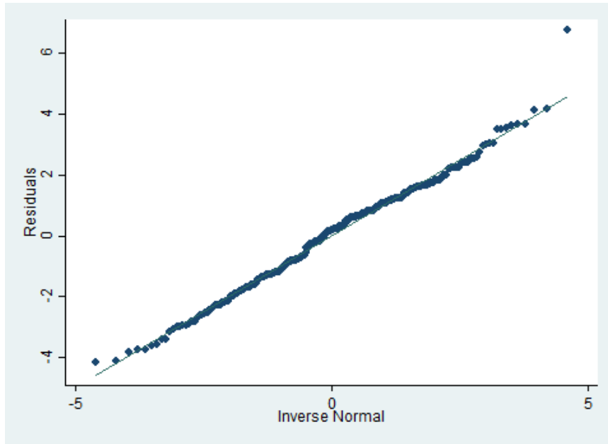
Supplementary file 2: Normality q-q plot
