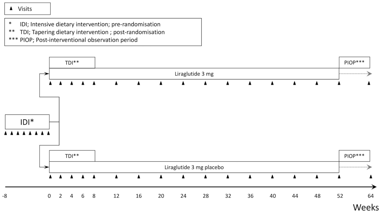
Figure 1 Trial design.
