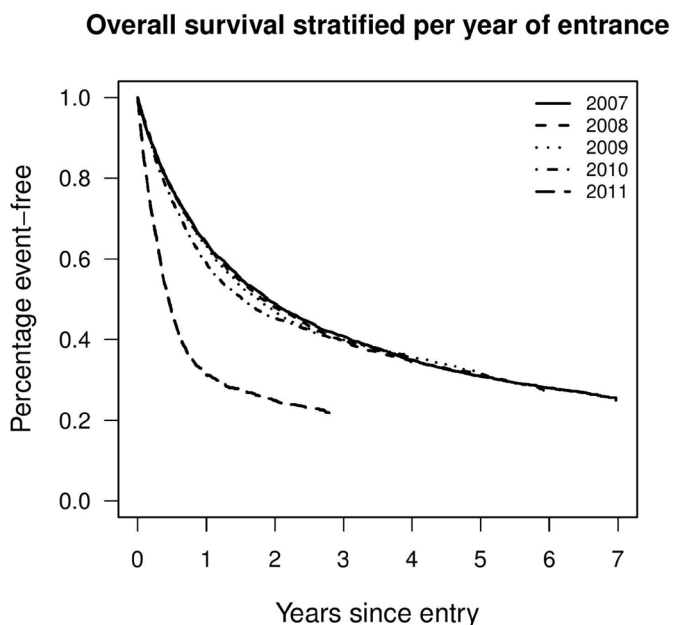
Figure 3 Kaplan-Meier estimator for the time in work disability, stratified by the year of entrance into work disability. Ending long-term work disability happens by death, retirement or ability to work, whichever occurs first.
