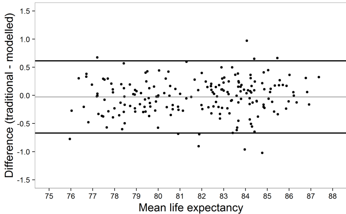
Supplementary Figure 1 Agreement between traditional and modelled life expectancy estimates. Differences are represented by filled circles, the thin grey line represents the marginal mean difference between estimates, and the thick black lines represent the upper and lower limits of agreement.
