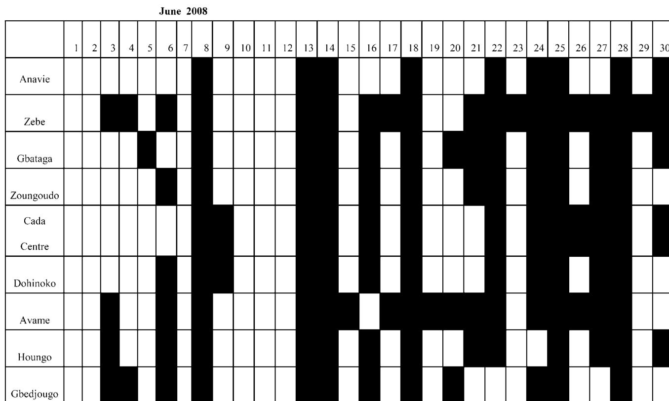
Figure 6 Number of rainy days per village in Tori Bossito (example of June 2008). Note: Black squares symbolise rainy days and white squares days with no rainfall.
