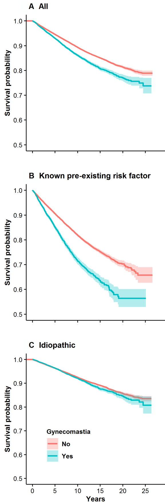
Figure 3 Kaplan-Meier plots of the time course of death, according to gynaecomastia (all gynaecomastia, with a known pre-existing recognised risk factor, idiopathic).
