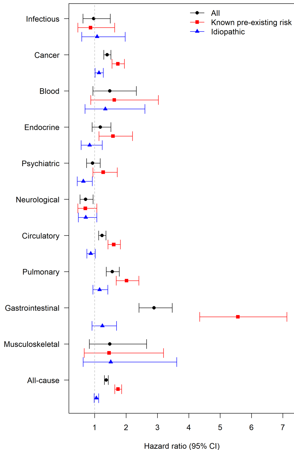
Figure 2 Death risks, all HRs and 95% CI for gynaecomastia (all, with a known pre-existing risk factor, idiopathic).
