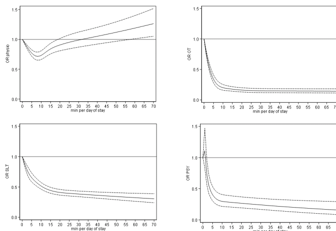
Figure 1 Cubic splines describing the Odds Ratio (95% CI) for disability on discharge per minute therapy/day of inpatient stay (referenced to zero). Top left to bottom right=physiotherapy; occupational therapy (OT); speech and language therapy (SLT); psychology (PSY).
