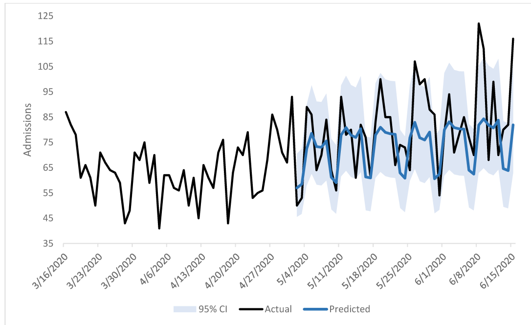
Figure A4.2: Forecast versus Actual values for June 2020 Horizon
