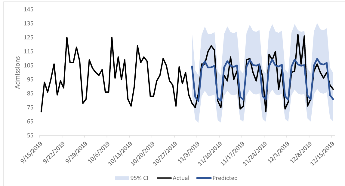
Figure A4.1: Forecast versus Actual values for December 2019 Horizon.
