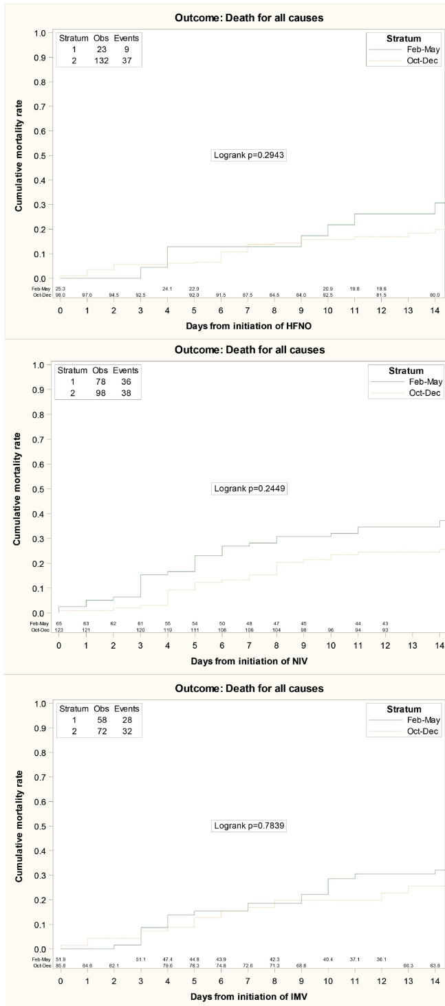
Supplementary Figure 3. Survival KM estimates stratified by pandemic wave, restricted to patients who required the use of respiratory support (HFNO, NIV and IMV)
