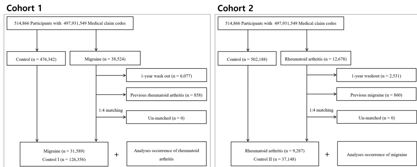
Figure 1 Schematic illustration of the participant selection process that was used in this study. Cohort 1: Of 514 866 participants, 31 589 migraine patients were matched with 126 356 control I participants for age group, sex, income group and region of residence. Cohort 2: Of 514 866 participants, 9287 rheumatoid arthritis patients were matched with 37 148 control II participants for age group, sex, income group and region of residence.
