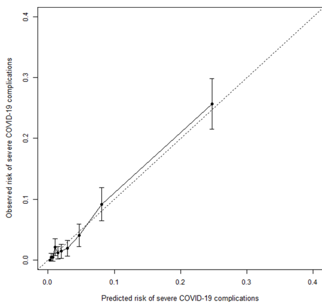
Figure 2 Calibration plot of least absolute shrinkage and selection operation (LASSO) regression of severe COVID-19 complications predicted by the sCOVID algorithm versus the observed complications. The Brier Score was 0.034. The calibration intercept was 0.09. The calibration slope was 1.04.
