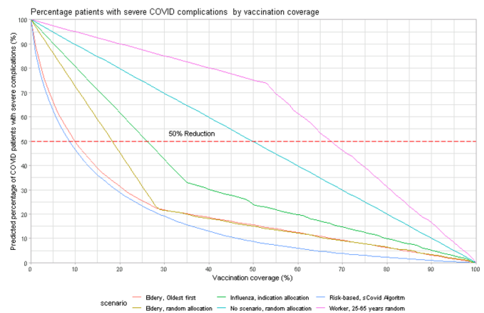
Figure 3 Effect of vaccination on the reduction of severe COVID-19 complications in different scenarios. Vaccination coverages needed for a 50% reduction of the burden of disease can be estimated at the intersection of the graphs with the 50% reduction line.
