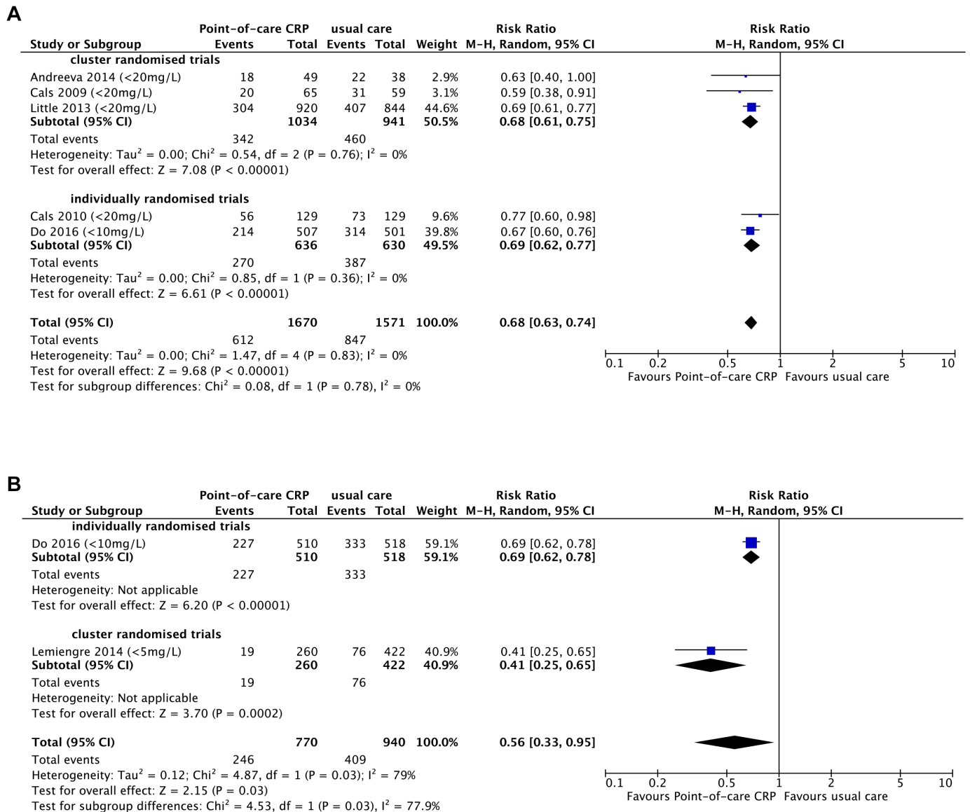
Figure 2 Forest plot of comparison: point-of-care CRP versus usual care, outcome: antibiotic prescribing at index consultation: (A) RCTs, adults only, if cut-off guidance applied; (B) RCTs, children only, if cut-off guidance applied. CRP cut-off used to withhold antibiotic treatment between brackets. CRP, C reactive protein; M-H, Mantel-Haenszel; RCTs, randomised controlled trials.
