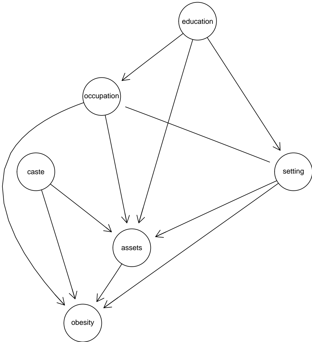
Fig.S1. Causal diagram created using Bayesian Network Learning
