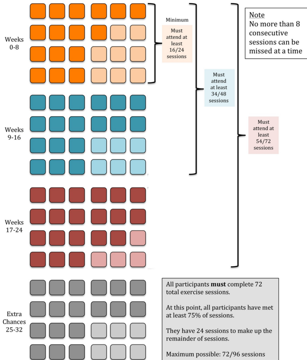
Figure 2 Adherence infographic.
